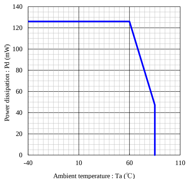
Ambient temp. vs. Power dissipation
