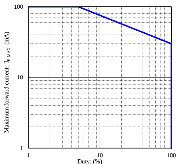
Duty cycle vs. Maximum forward current
