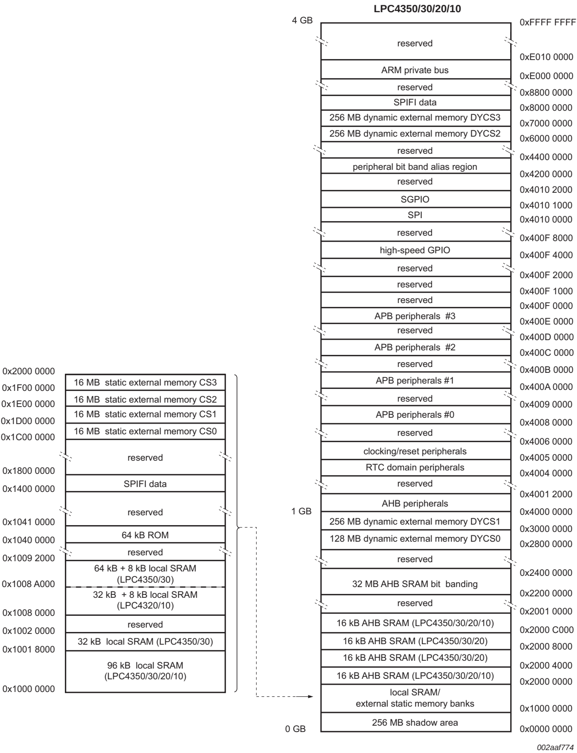
Fig 7. LPC4350/30/20/10 Memory mapping (overview)
