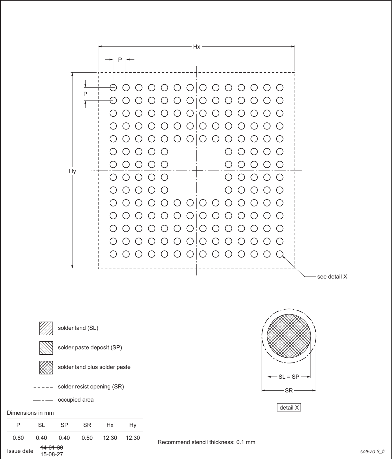
Footprint information for reflow soldering of TFBGA180 package SOT570-3
