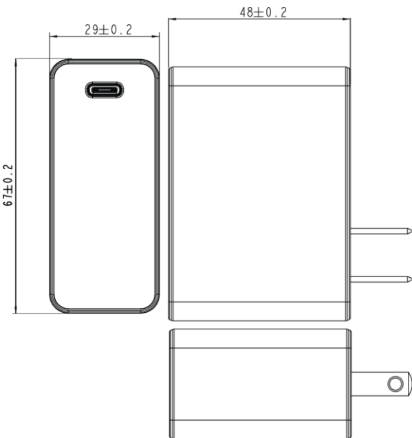
AQ36A-5CA-H Dimension Diagram Unit: mm
