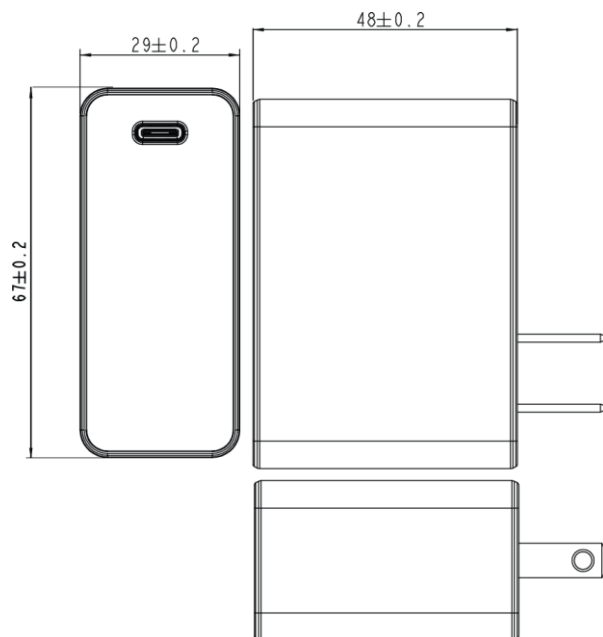
AQ36A-5CA-H Dimension Diagram Unit: mm
