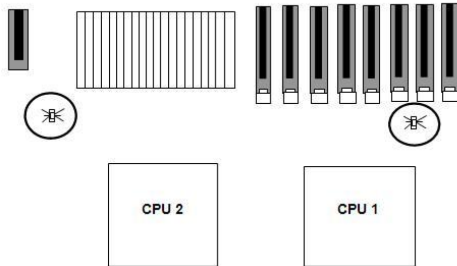
Figure 13. Processor Fault LED Locations
