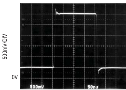
Large Signal Response V_S = 5V, 0V
