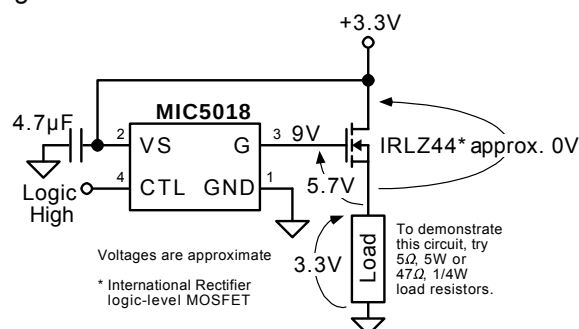
Figure 3. Using a Logic-Level MOSFET
