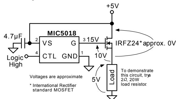
Figure 2. Using a Standard MOSFET
