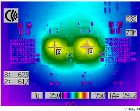
Figure 4. Thermal Capture at 12V IN , 1.8V OUT , 30A, 500kHz No Forced Airflow (Convection). T A = 29°C.
