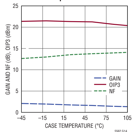
Conversion Gain, OIP3 and NF vs Case Temperature
