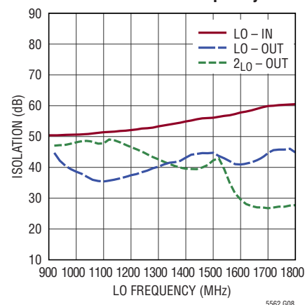
LO Isolation vs LO Frequency
