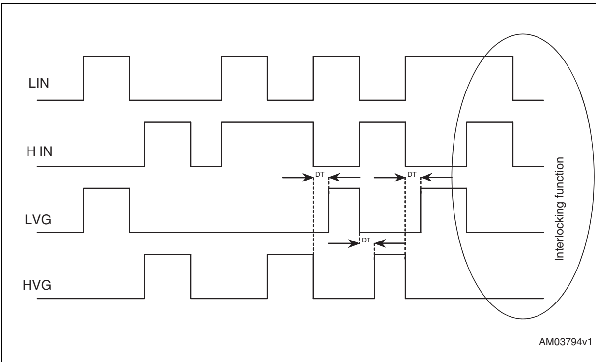
Figure 9. Dead time and interlocking definition
