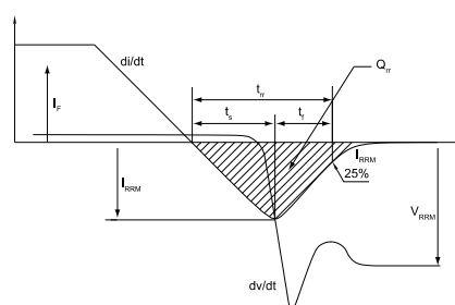
Figure 22: Diode reverse recovery waveform
