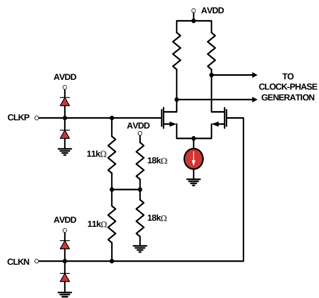
FIGURE 44. CLOCK INPUTS
