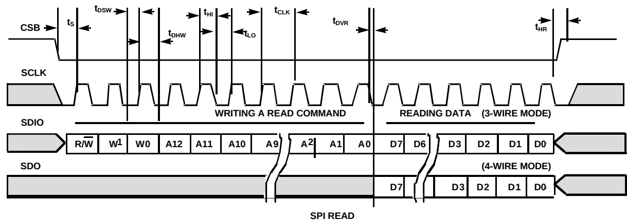
FIGURE 39. SPI READ
