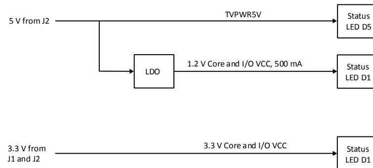
Figure 4.1. Power Supply
