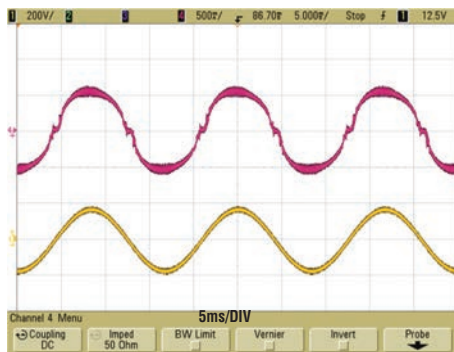
Figure 5. 120VAC (PF = 0.99)
