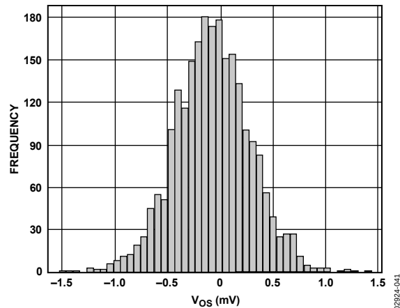
Figure 41. Initial Offset
