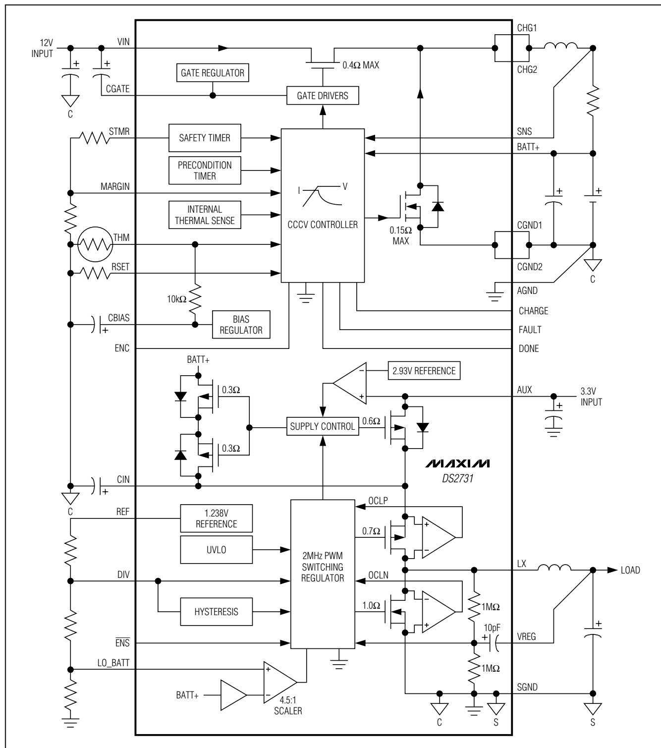
Figure 2. Block Diagram
