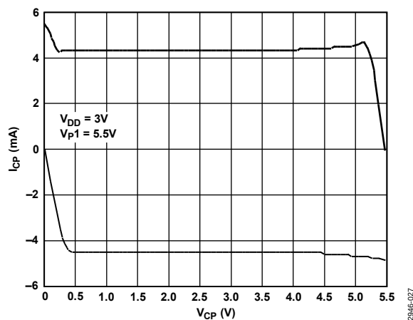
Figure 26. RF Charge Pump Output Characteristics
