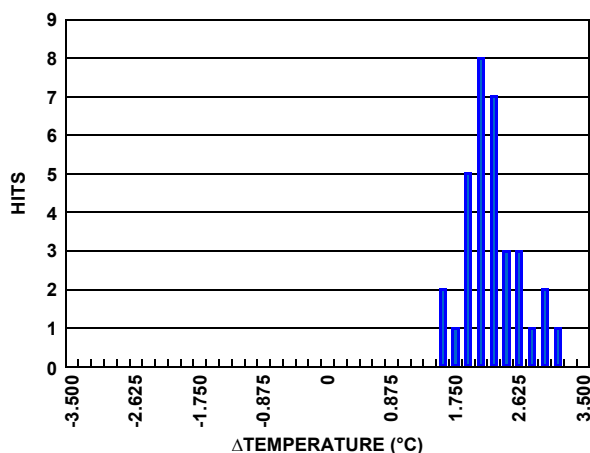
FIGURE 53. INTERNAL TEMPERATURE ACCURACY AT T = +85^\circ\text{C}
