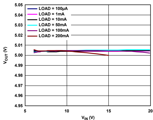
Figure 6. Output Voltage ( V_{OUT} ) vs. Input Voltage ( V_{IN} )
