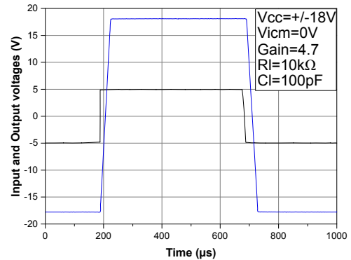
Figure 28. Output desaturation vs. time
