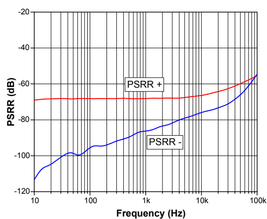
Figure 34. PSRR vs. frequency at V_{CC} = 36\text{ V}
