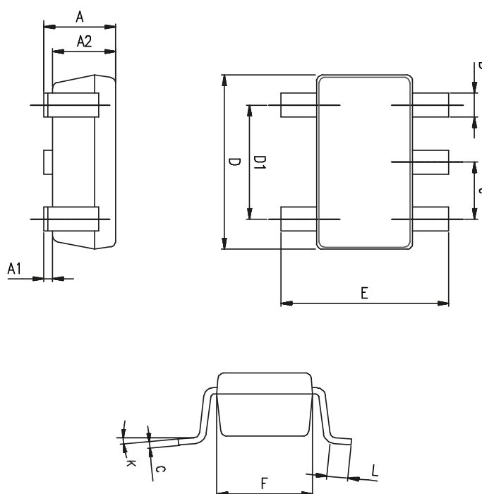
Figure 39. SOT23-5 package outline
