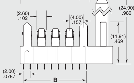
EBTM-4-10-2.0-S-VT-1-L-G SHOWN
