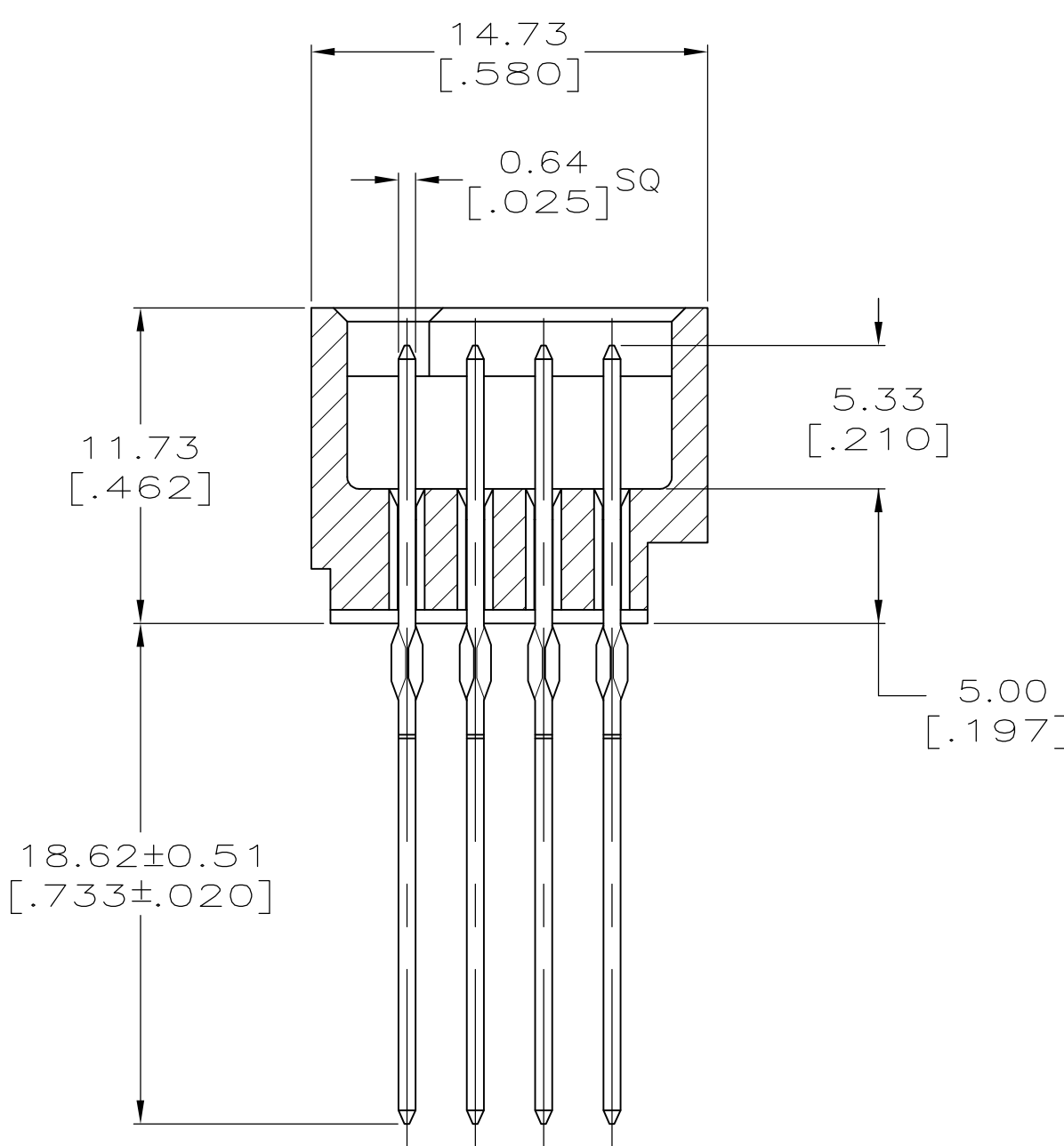
SECTION T-T
