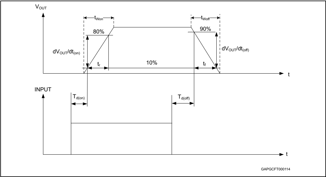
Figure 8. Switching characteristics
