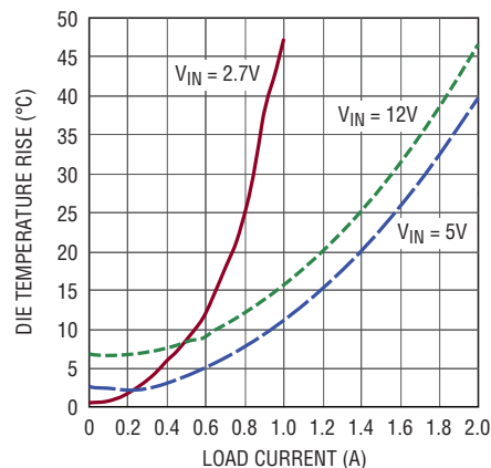
3.3V _{OUT} Die Temperature Rise vs Continuous Load Current 4-Layer Demo Board at 25^\circ\text{C}
