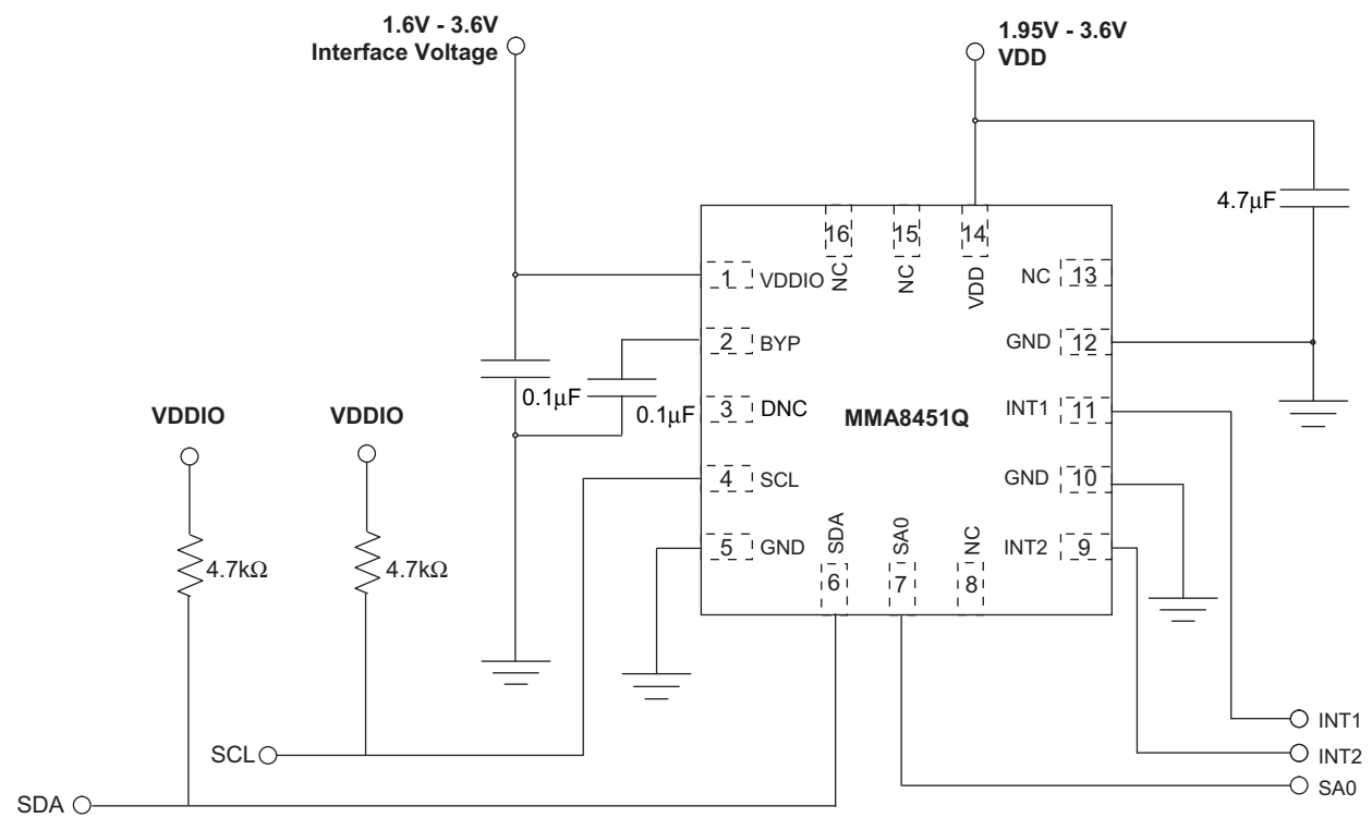
Figure 4. Application diagram
