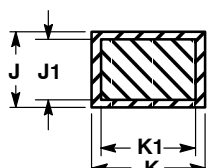
SECTION N-N
