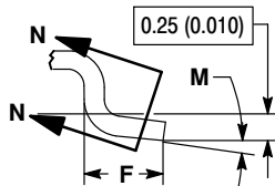
DETAIL E
