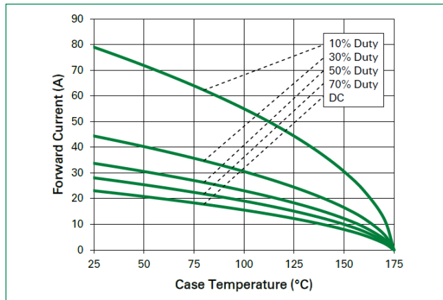
Figure 4: Current Derating
