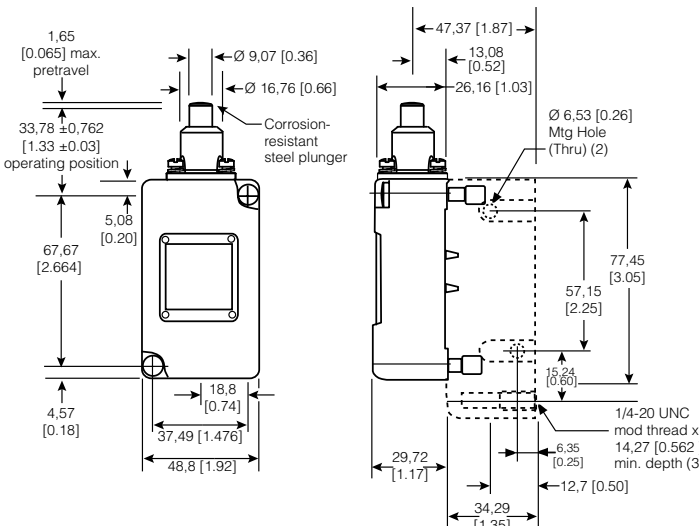
Figure 16. 203LS1 Dimensions
