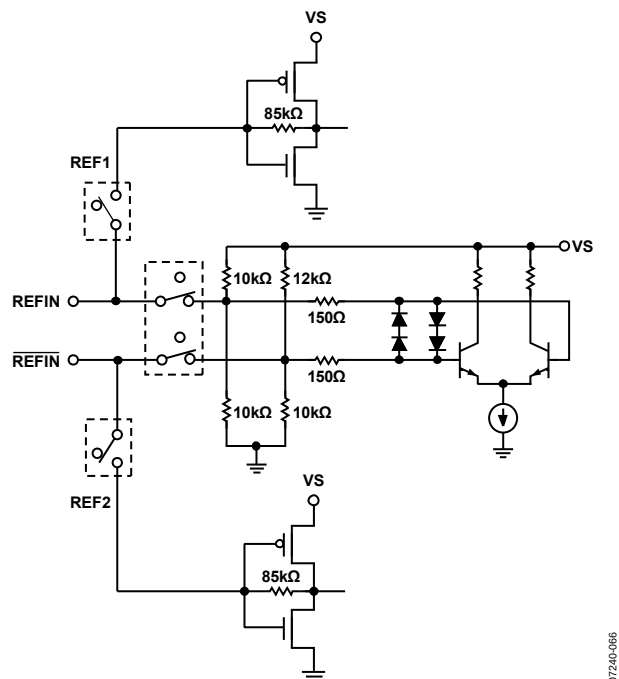
Figure 30. REF1 Equivalent Circuit for Non-XTAL Mode
