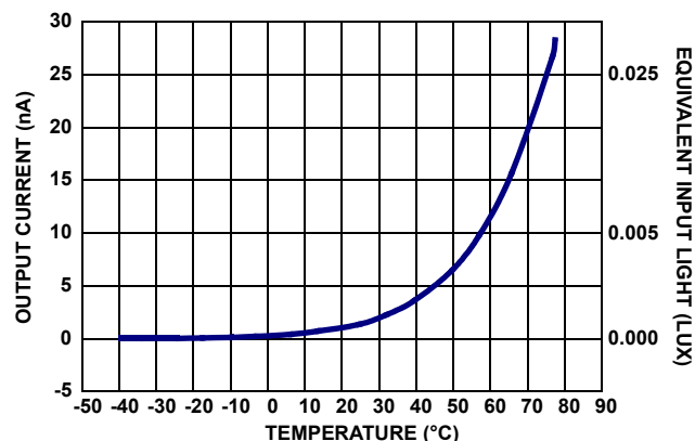
FIGURE 11. OUTPUT CURRENT vs TEMPERATURE AT 0 LUX
