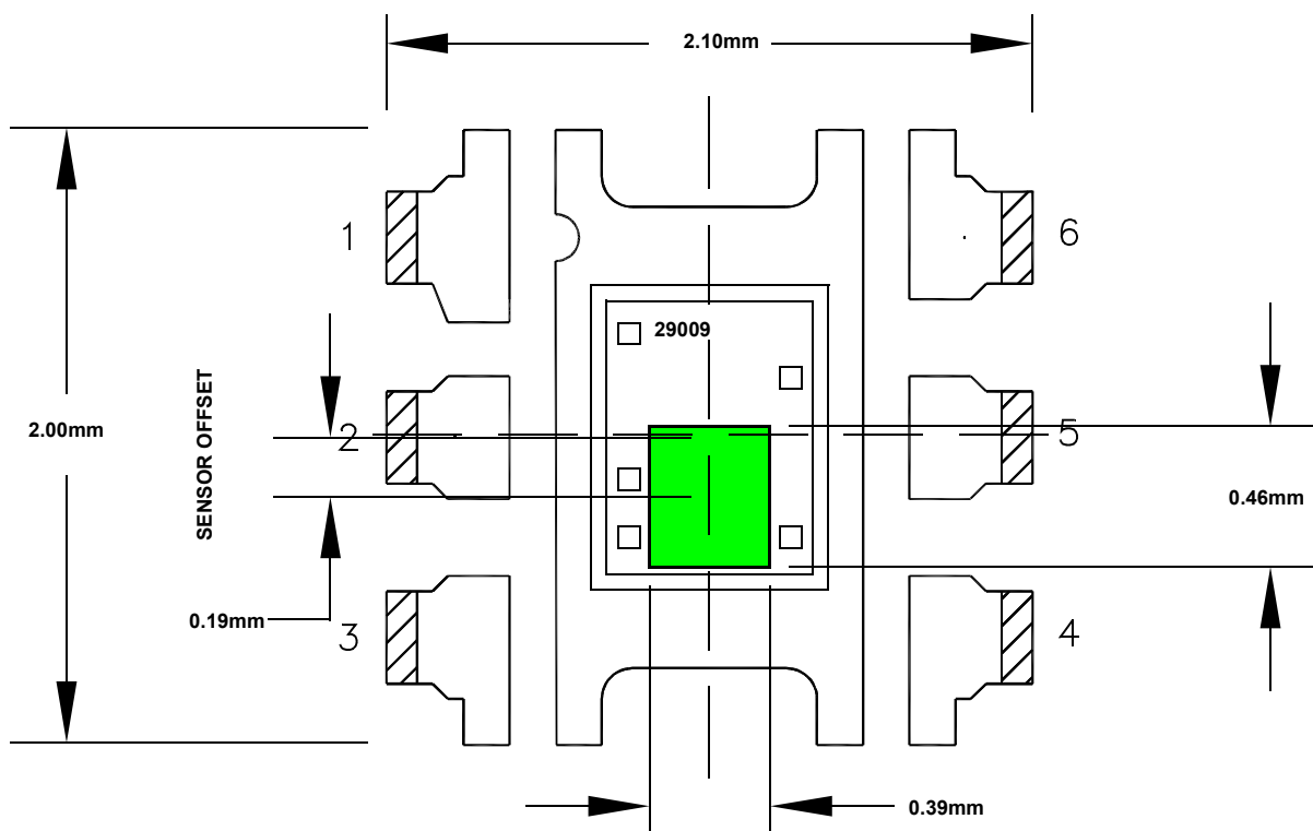
FIGURE 18. 6 LD ODFN SENSOR LOCATION OUTLINE
