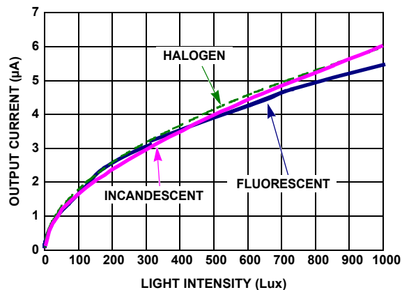
FIGURE 7. OUTPUT CURRENT vs LIGHT INTENSITY
