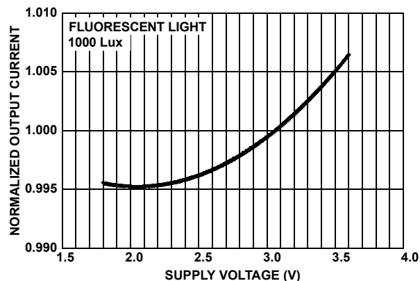
FIGURE 15. NORMALIZED OUTPUT CURRENT vs SUPPLY VOLTAGE
