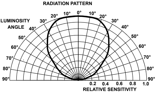
FIGURE 5. RADIATION PATTERN
