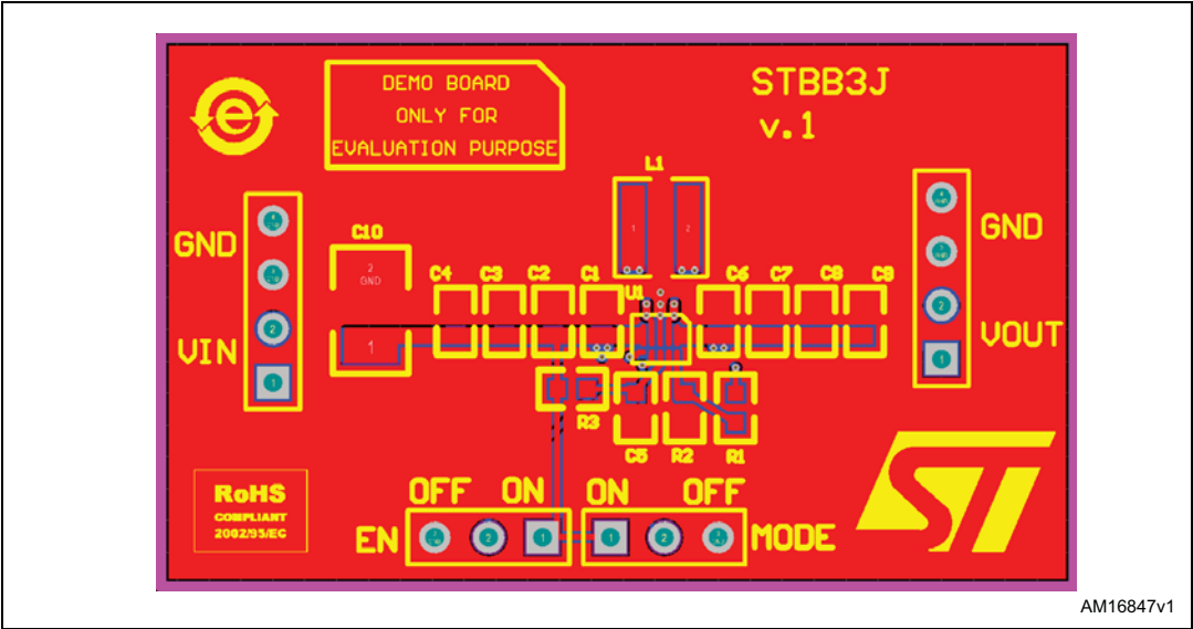
Figure 33. Top layer
