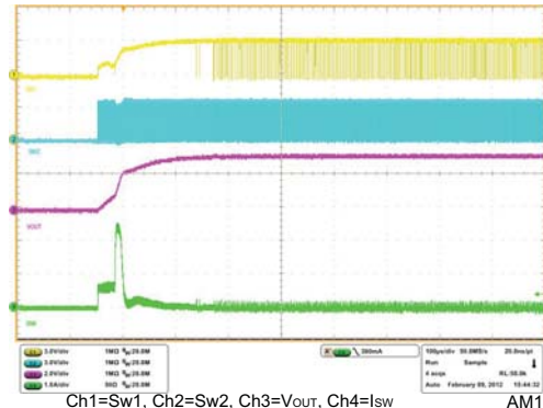
Figure 22. Startup after enable @ V_{IN}=3.6\text{ V}
