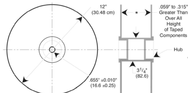
Figure 3: Standard Reel
