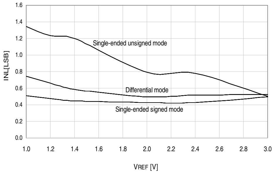
Figure 34-166. INL error vs. external V_{REF} .
