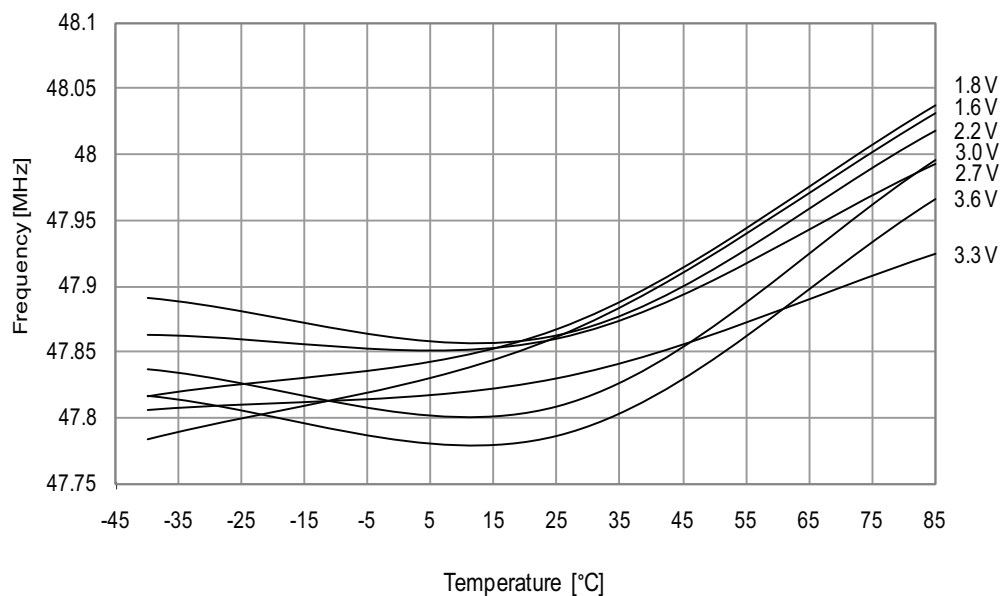
Figure 34-133. 48MHz internal oscillator frequency vs. temperature. DPLL enabled, from the 32.768kHz internal oscillator.
