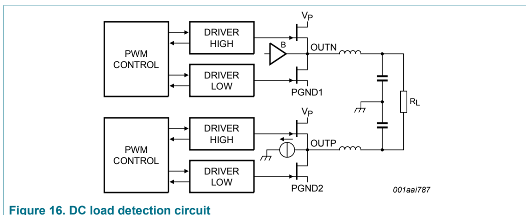
Figure 16. DC load detection circuit
