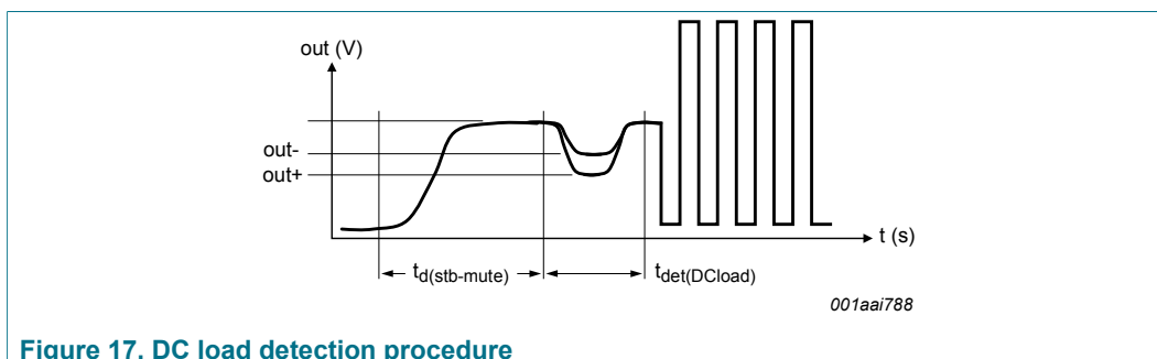
Figure 17. DC load detection procedure
