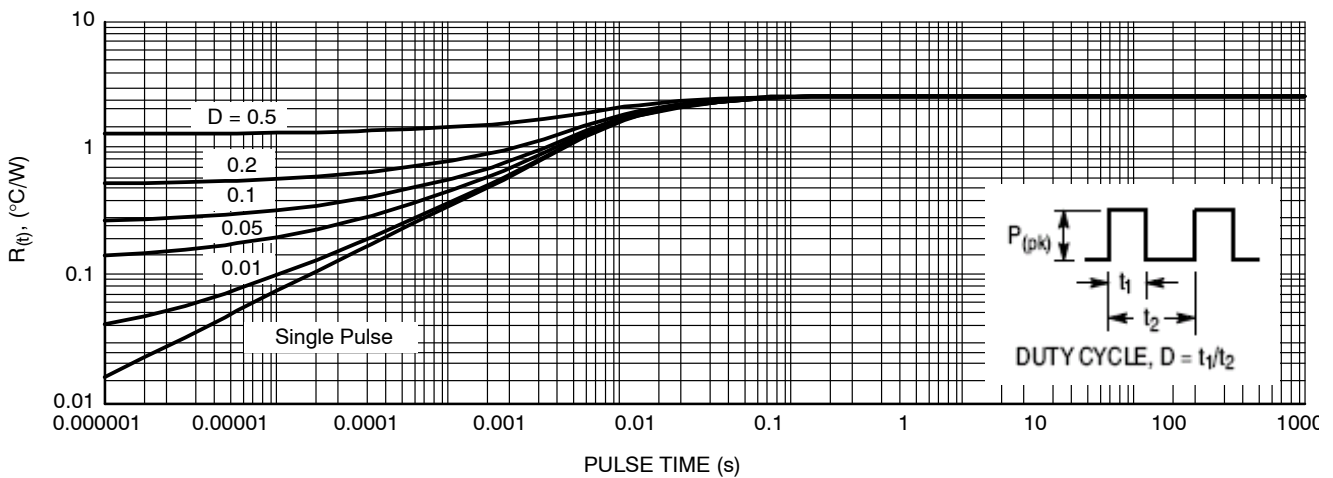
Figure 9. R_{\theta J} on an Infinite Heatsink Power (J1) 0.800 W Power (J2) 0.800 W
