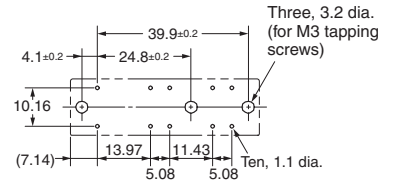
Mounting Hole Placement (Bottom View) (±0.1 tolerance)
