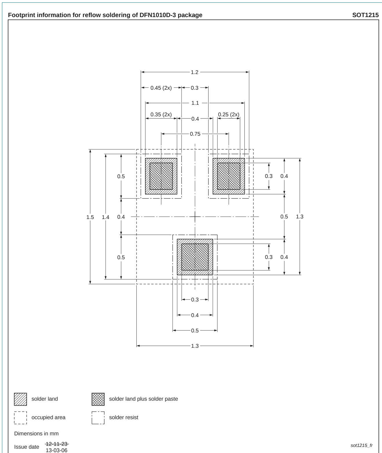
Fig 34. Reflow soldering footprint DFN1010D-3 (SOT1215)
