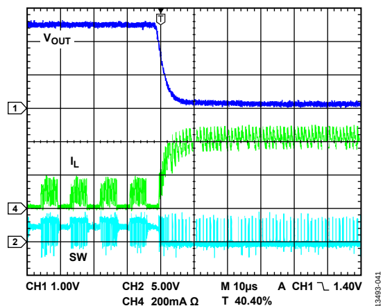
Figure 22. Output Short Protection
