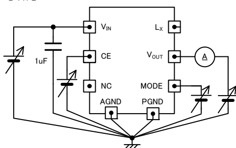
< Circuit ⑦ >
