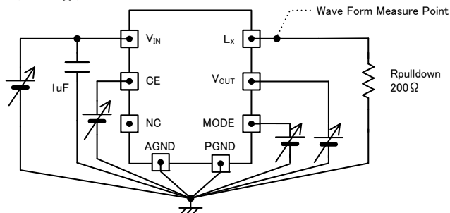
< Circuit ③ >
