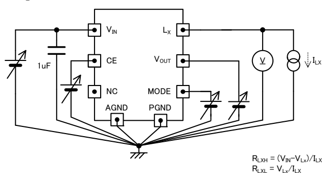
< Circuit ⑥ >
