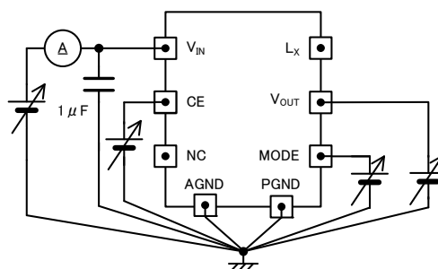
< Circuit ② >
