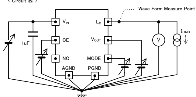
< Circuit ⑥ >
