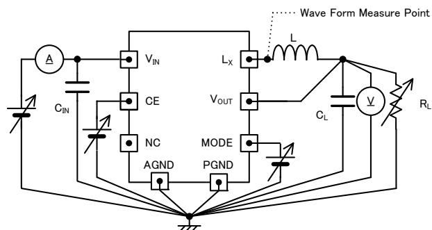
< Circuit ① >
