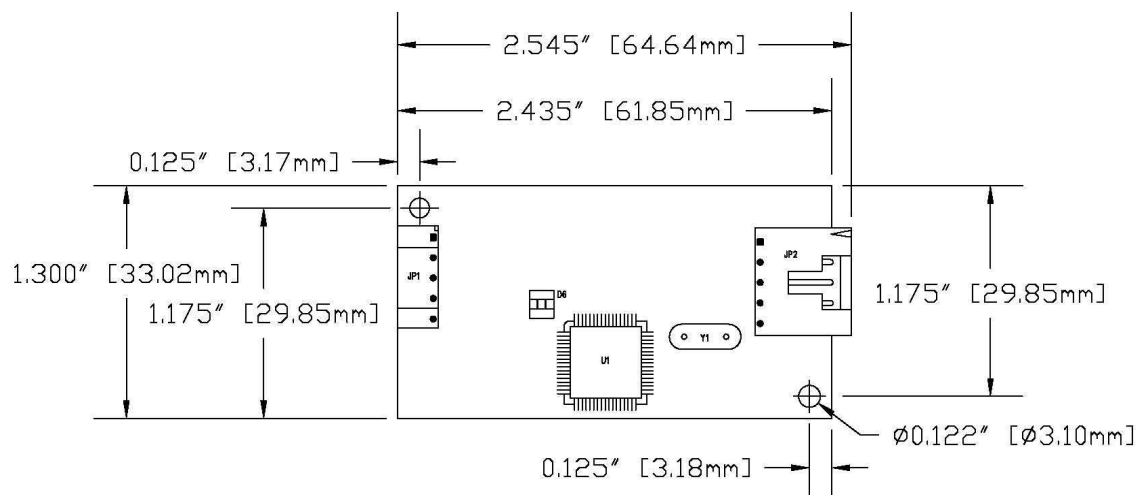
Figure 3 EX111 Dimensions
