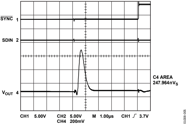
Figure 4. Digital-to-Analog Glitch Impulse Without Internal Deglitcher
