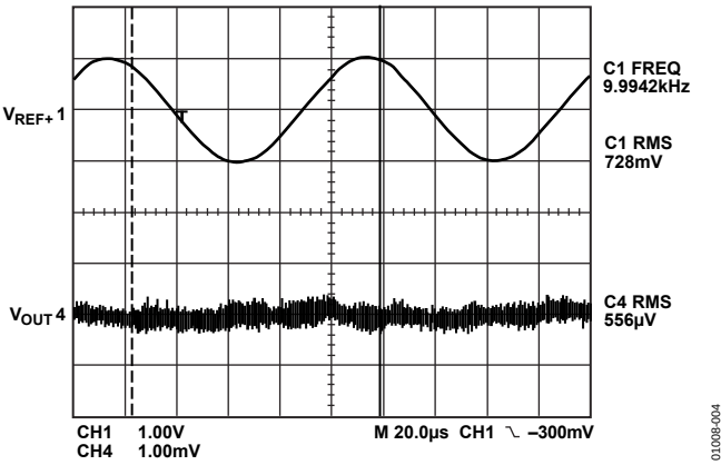
Figure 3. AC Feedthrough
