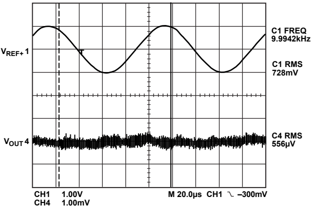
Figure 3. AC Feedthrough
