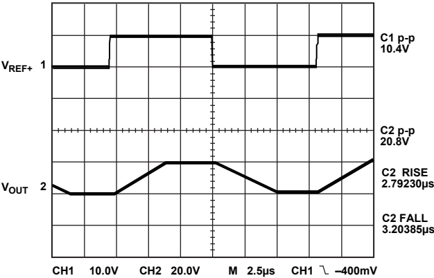
Figure 8. Pulse Response (Large Signal)
