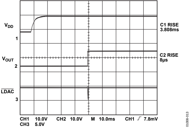
Figure 12. Turn-On Characteristics
