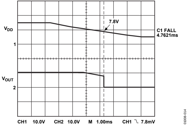
Figure 13. Turn-Off Characteristics
