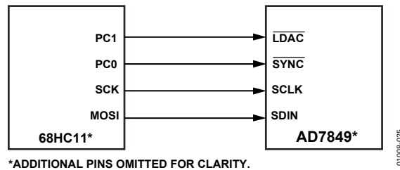
Figure 26. AD7849-to-68HC11 Interface
