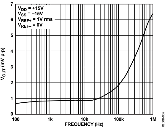
Figure 6. AC Feedthrough vs. Frequency
