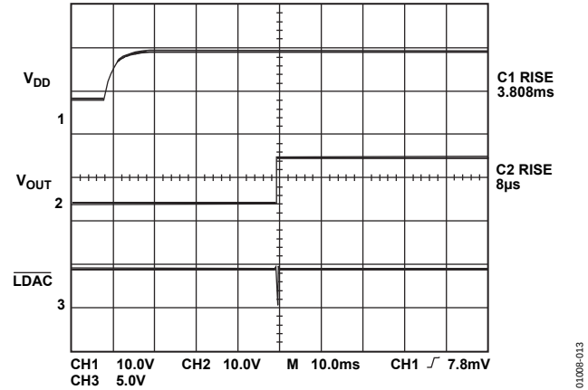
Figure 12. Turn-On Characteristics
