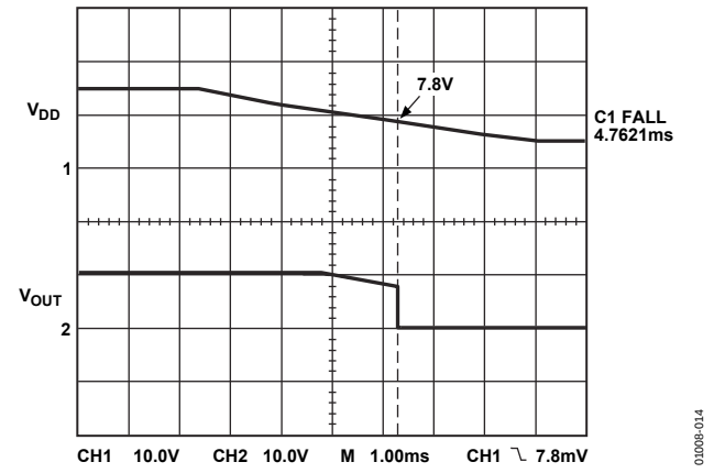
Figure 13. Turn-Off Characteristics
