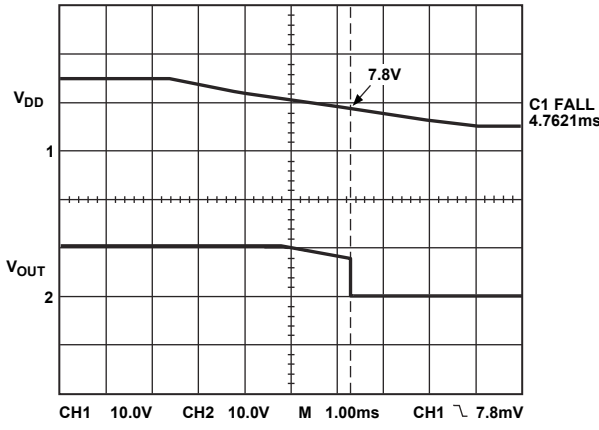
Figure 13. Turn-Off Characteristics
