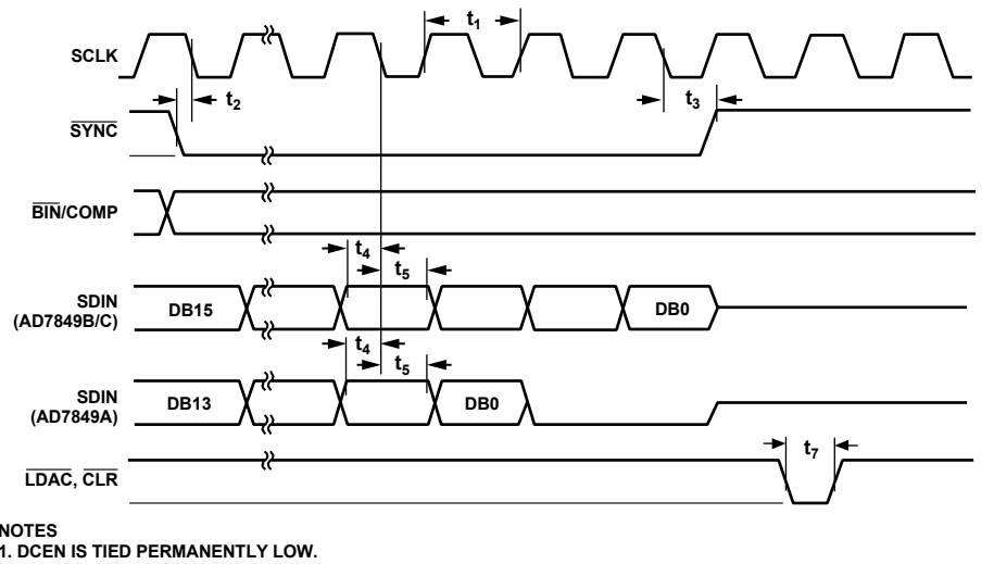
Figure 16. Timing Diagram (Standalone Mode)
