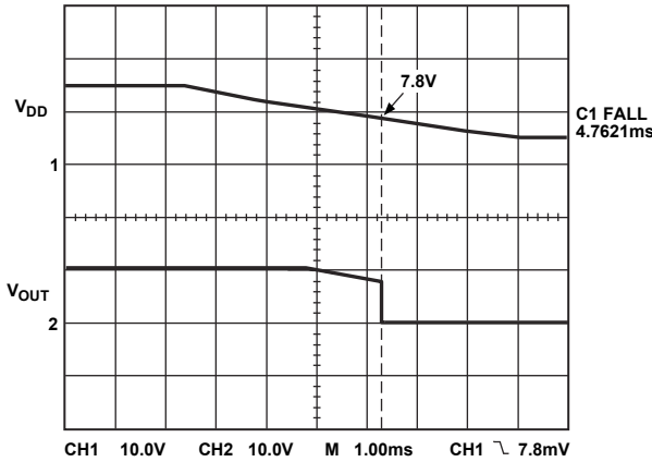
Figure 13. Turn-Off Characteristics
