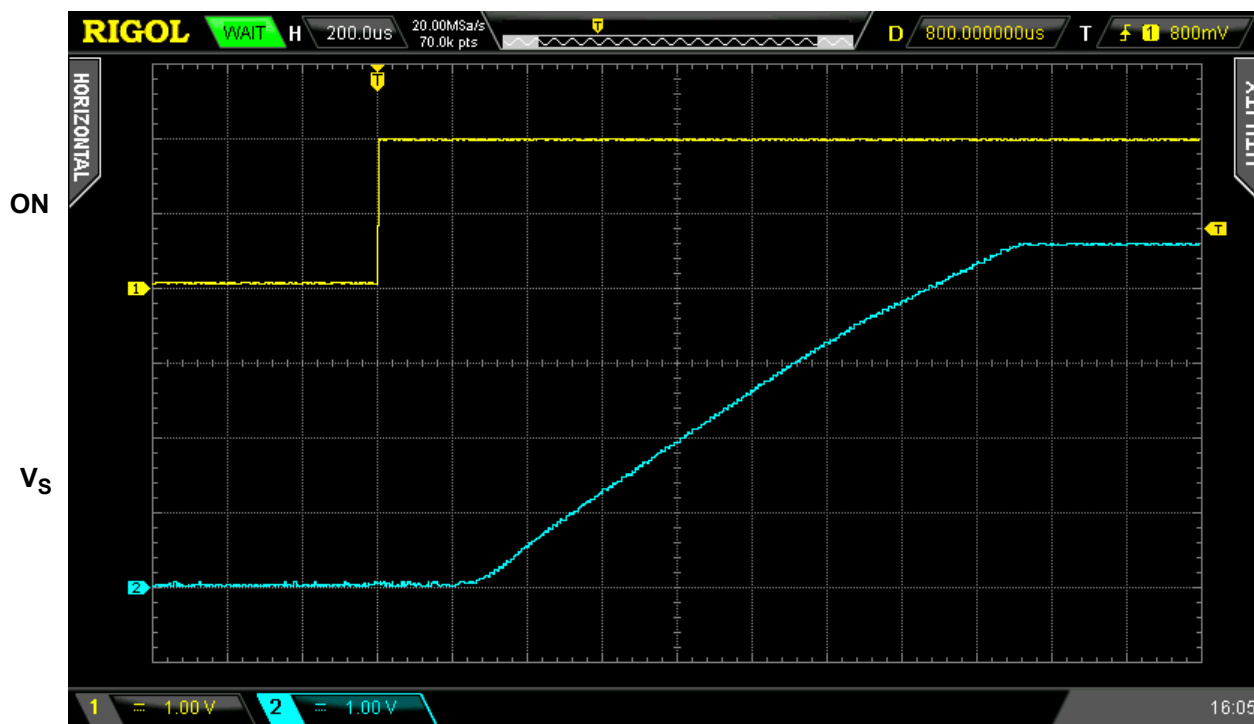
Figure 1. Typical Turn ON operation waveform for V_{IN} = 4.5\text{ V} , C_{SLEW} = 10\text{ nF} , C_{LOAD} = 10\text{ μF} , R_{LOAD} = 100\text{ Ω}
