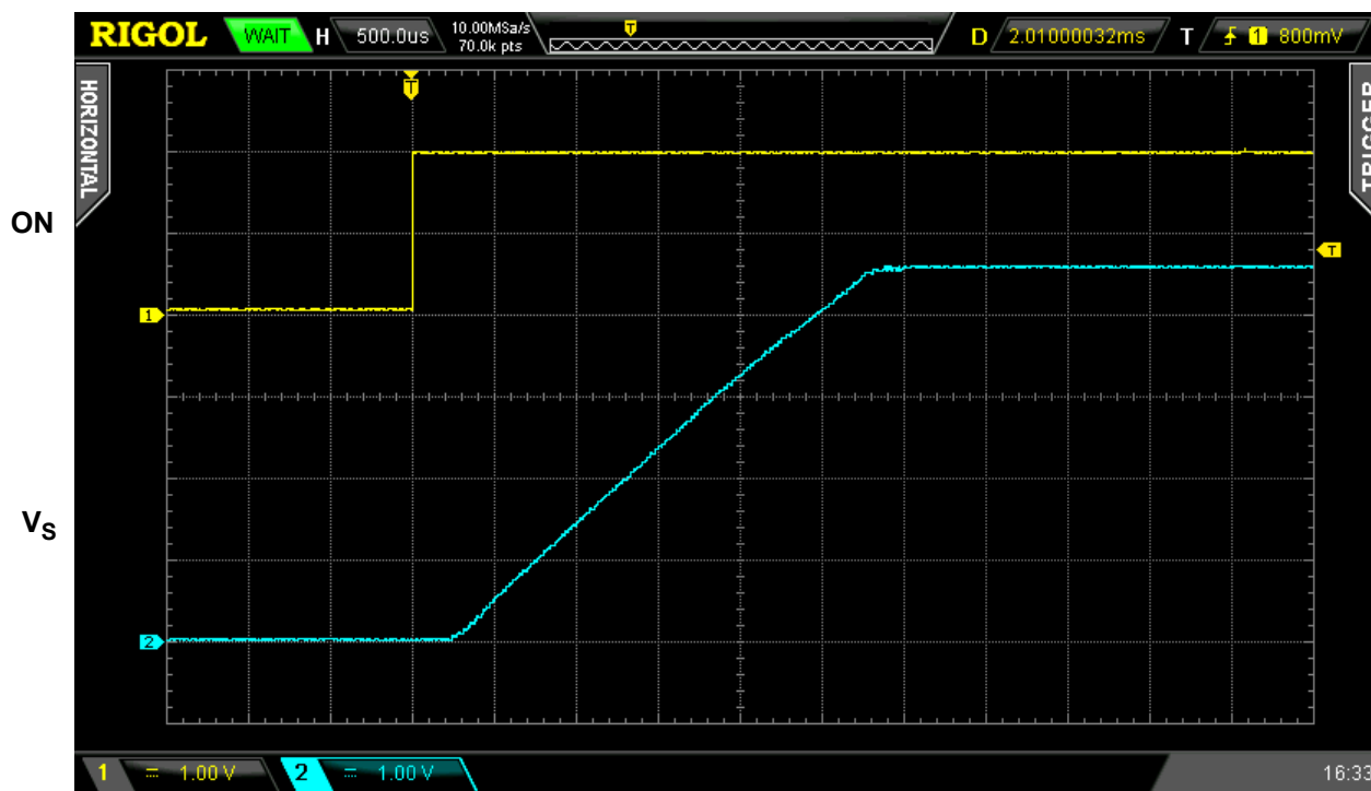
Figure 2. Typical Turn ON operation waveform for V_{IN} = 4.5\text{ V} , C_{SLEW} = 18\text{ nF} , C_{LOAD} = 10\text{ μF} , R_{LOAD} = 100\text{ Ω}
