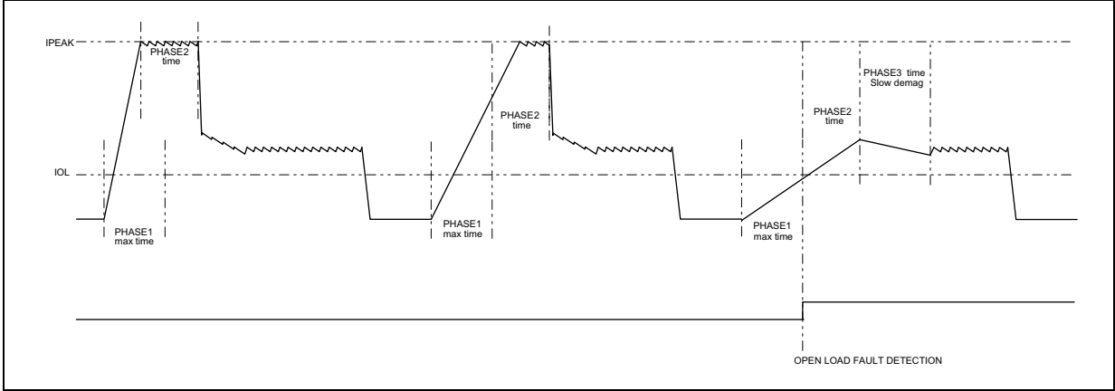
Figure 9. Open-load diagnostic
