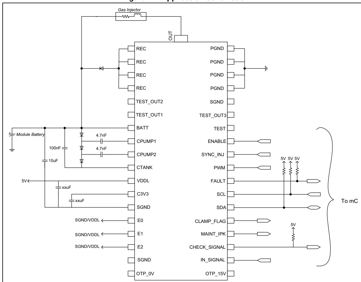
Figure 21. Application schematic
