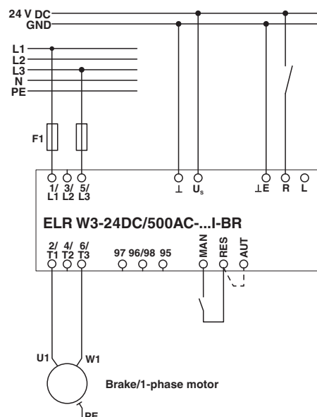
Circuit diagram
